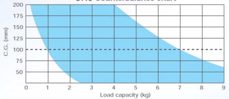
CH3 Counterbalance chart
