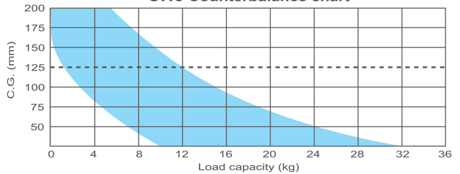
CH6 Counterbalance chart
