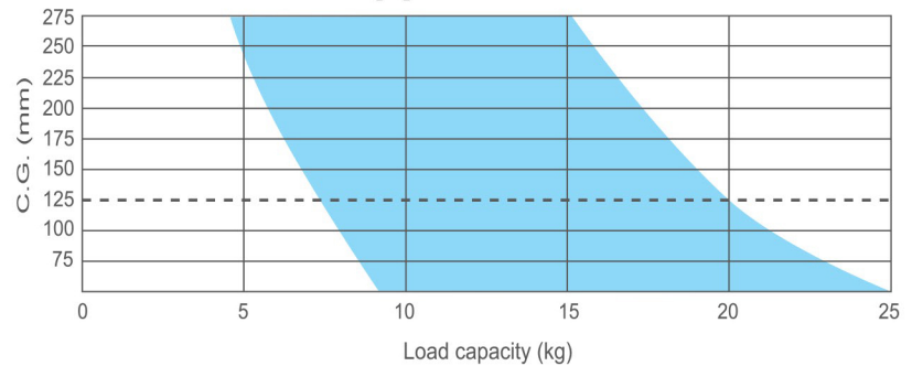
CH8(F) Counterbalance chart
