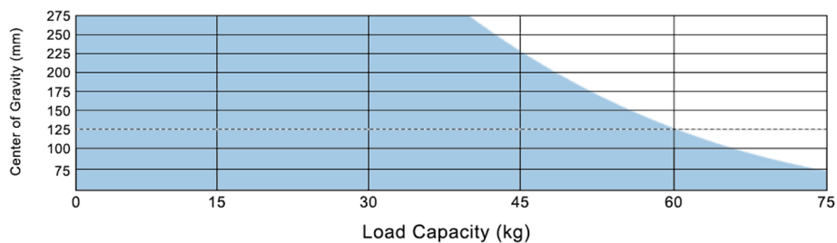
CINE90 Counterbalance Chart
