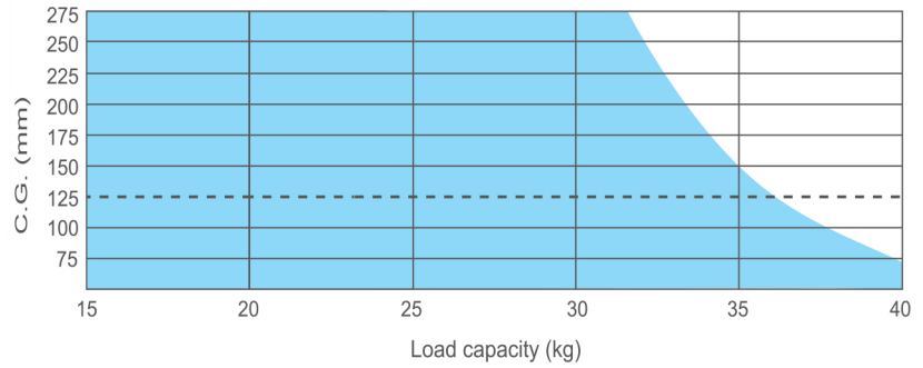
CHX(F) Counterbalance chart
